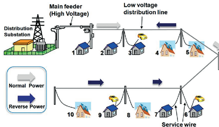
Fig 2.23: Low-voltage Distribution Network
