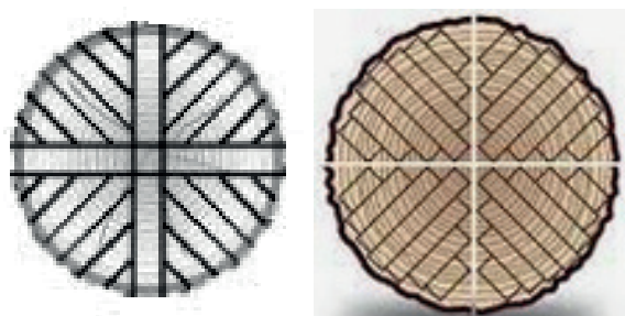
Fig 3.8: Quarter sawing
