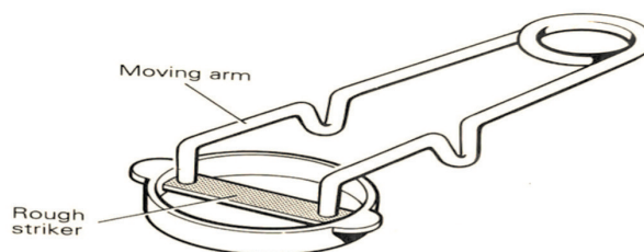
Fig. 3.21: Spark lighter.
