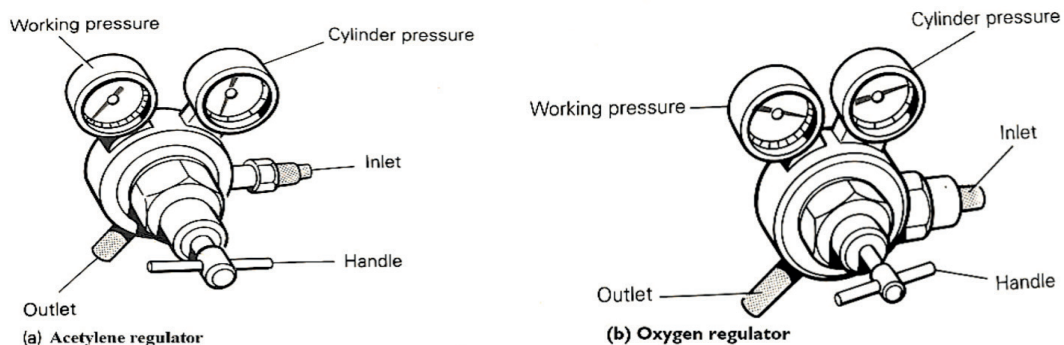
Fig. 3.18: Pressure regulators.
