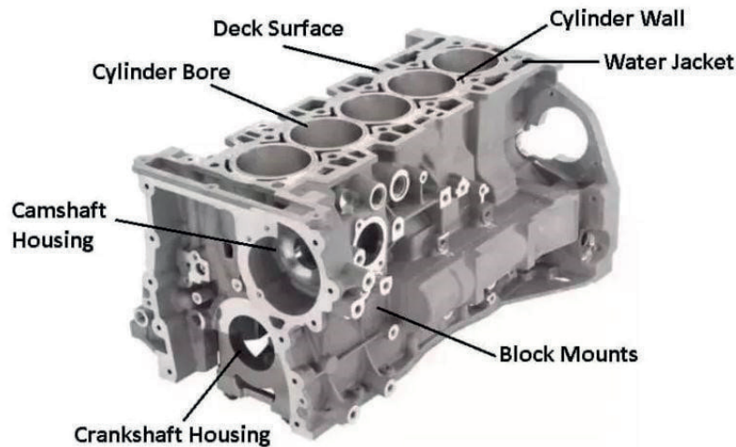
Fig 1.12: Cylinder block
