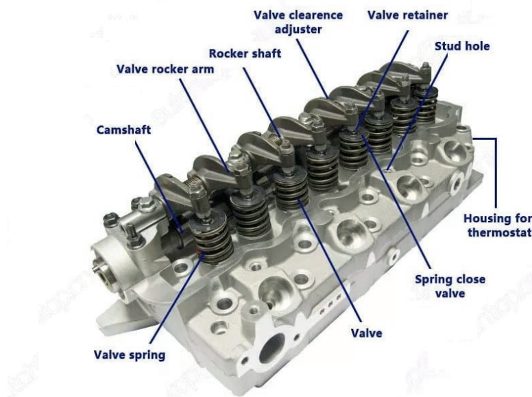
Fig 1.13: Cylinder head
