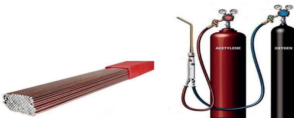
Fig. 3.22: Oxyacetylene equipment set-ups.
