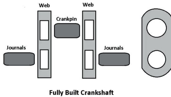
Fig. 1.9: Fully Built (Source: Fully Built Crankshaft - Search Images (bing.com))
