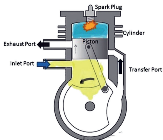
Fig 2.12: two-stroke cycle.
