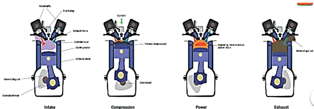
Fig 2.9: Petrol engines
