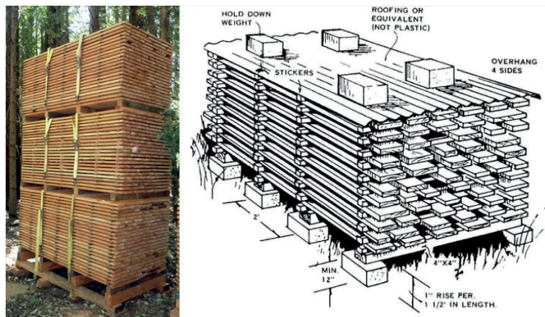
Fig 3.9: Timber air drying method.
