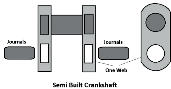
Fig. 1.10: Semi Built Crankshaft (source: Semi Built Crankshaft - Search Images (bing.com))
