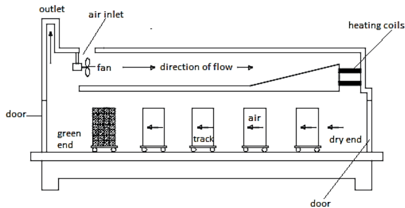
Fig 19: Progressive kiln.
