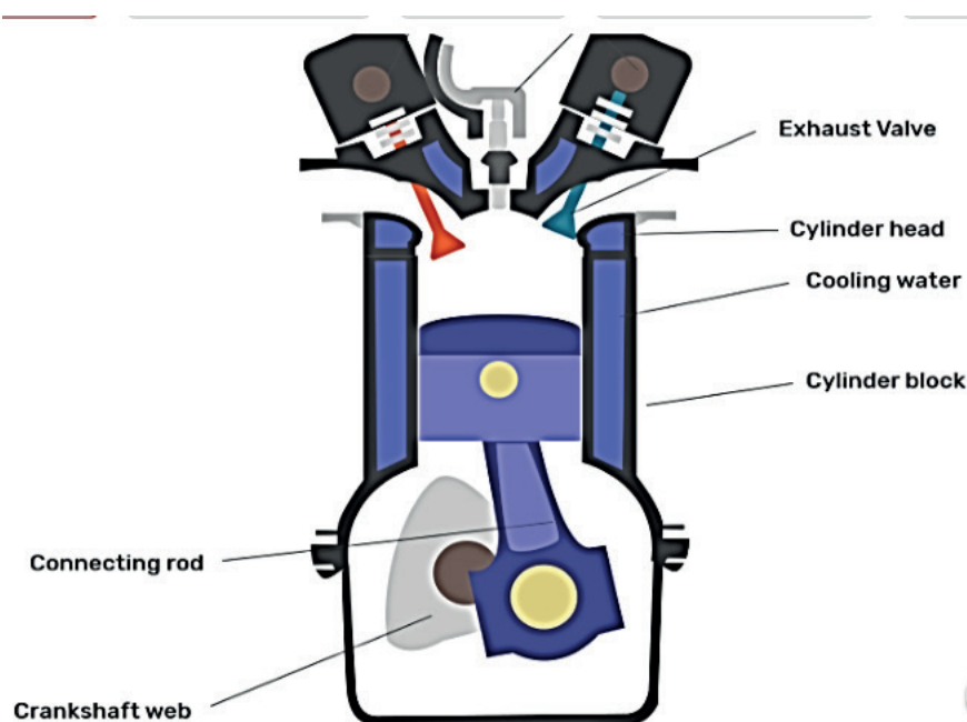
Fig 2.8: Petrol engine at fuel inlet position.
