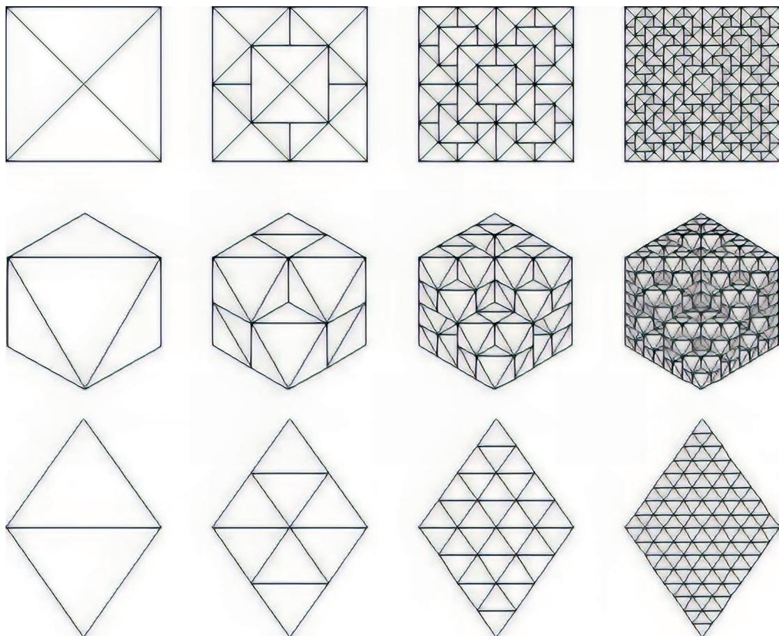
Figure. 2.3.1: Kepler's fractals
