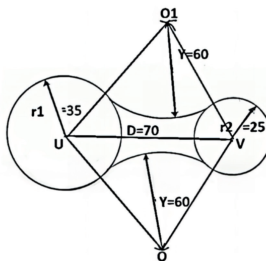
Figure 2.1.8: Blending of two circles internally.
