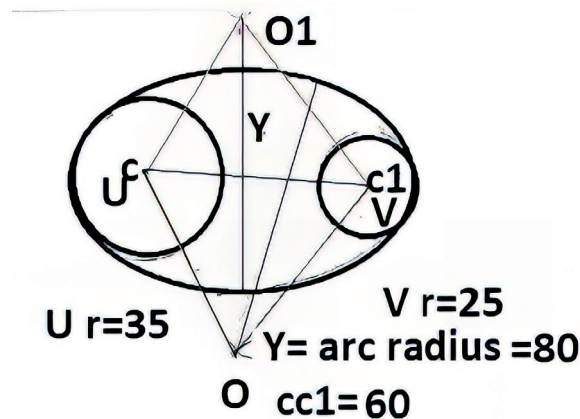
Figure 2.1.11: Blending of two circles of different radii externally
