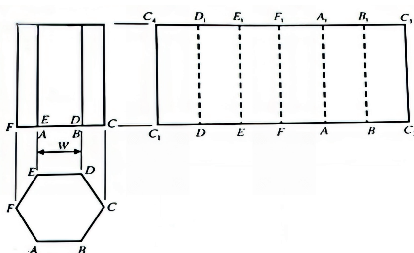
Figure 2.2.11: Hexagonal prism
