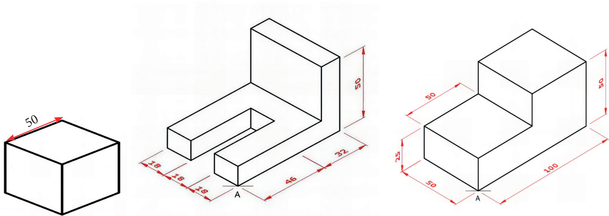
Figure 2.2.9: Isometric blocks
