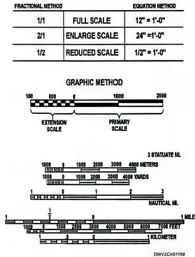
Figure 1.3.5: Scale Template
