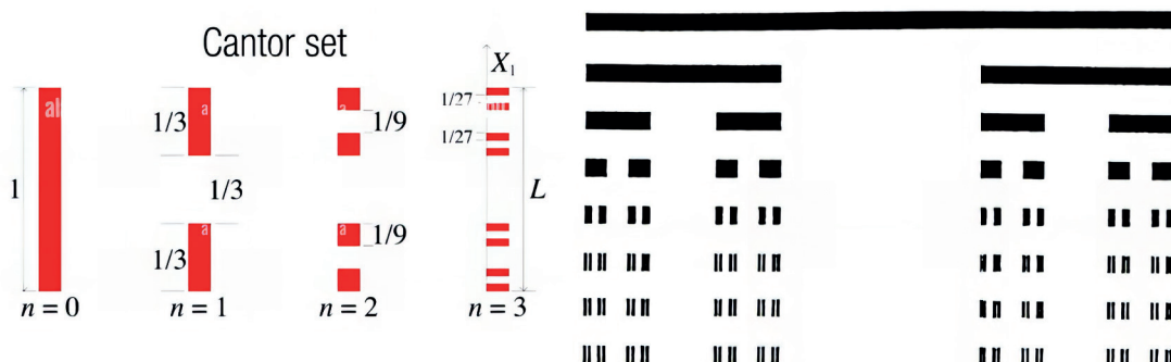
Figure. 2.3.5: Cantor set
